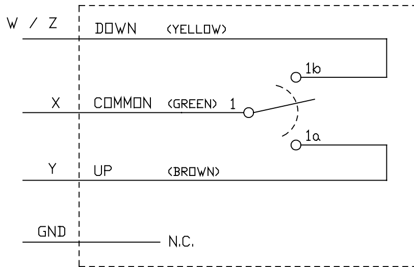
4 PIN (2411) POCKET PICKLE WIRING DIAGRAM
