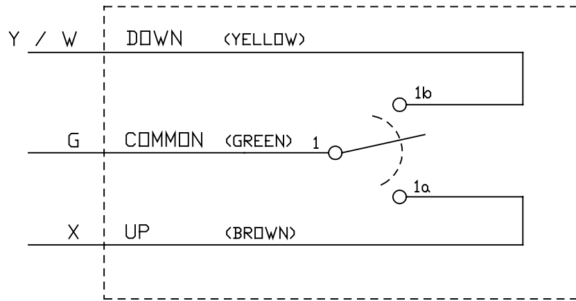
3 PIN (2311) POCKET PICKLE WIRING DIAGRAM
